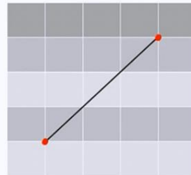
Euclidean Distance
